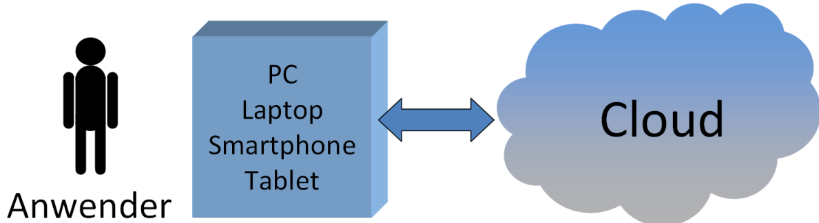
Abb. 1: Cloud Computing
